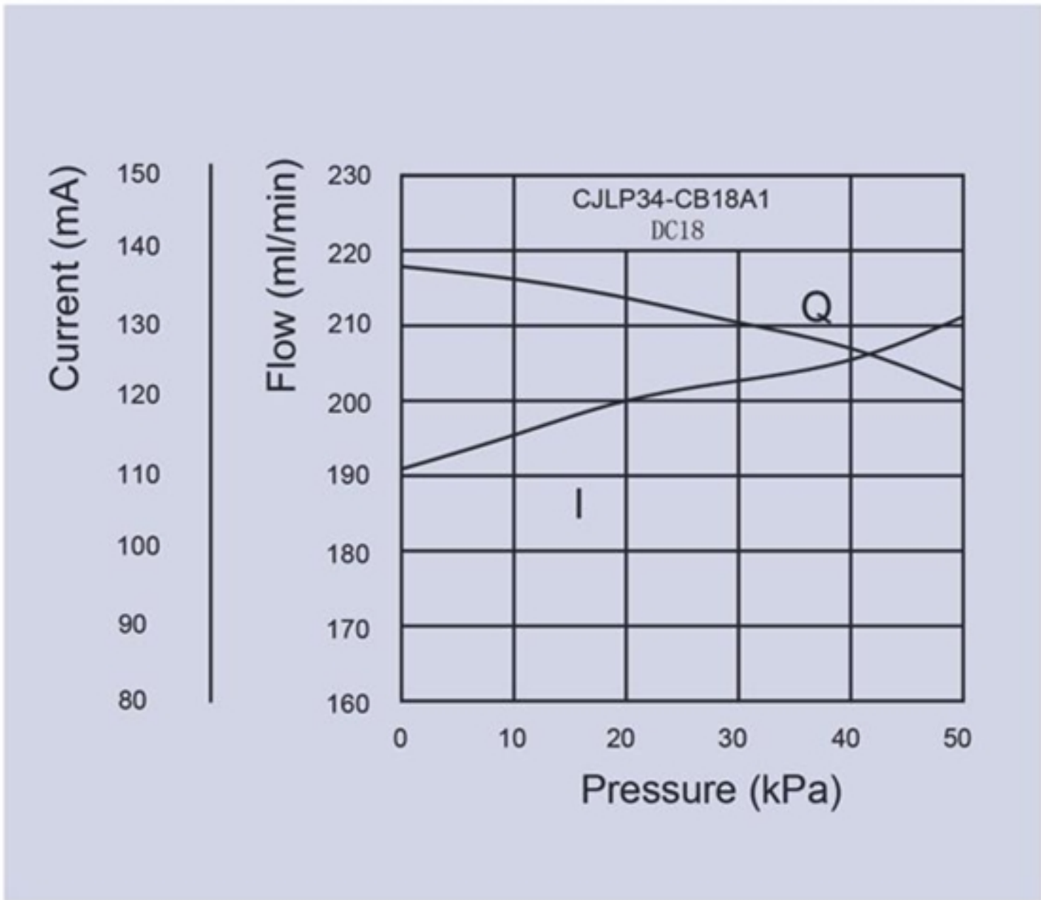
產品特性圖 Performance Curve
