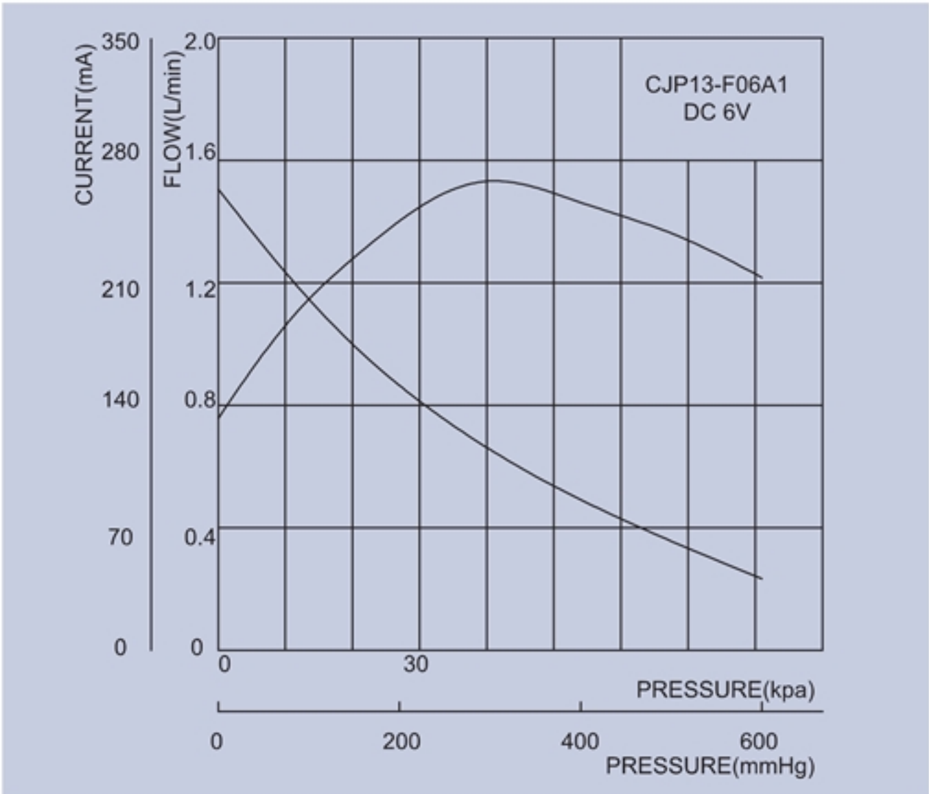
產品特性圖 Performance Curve
