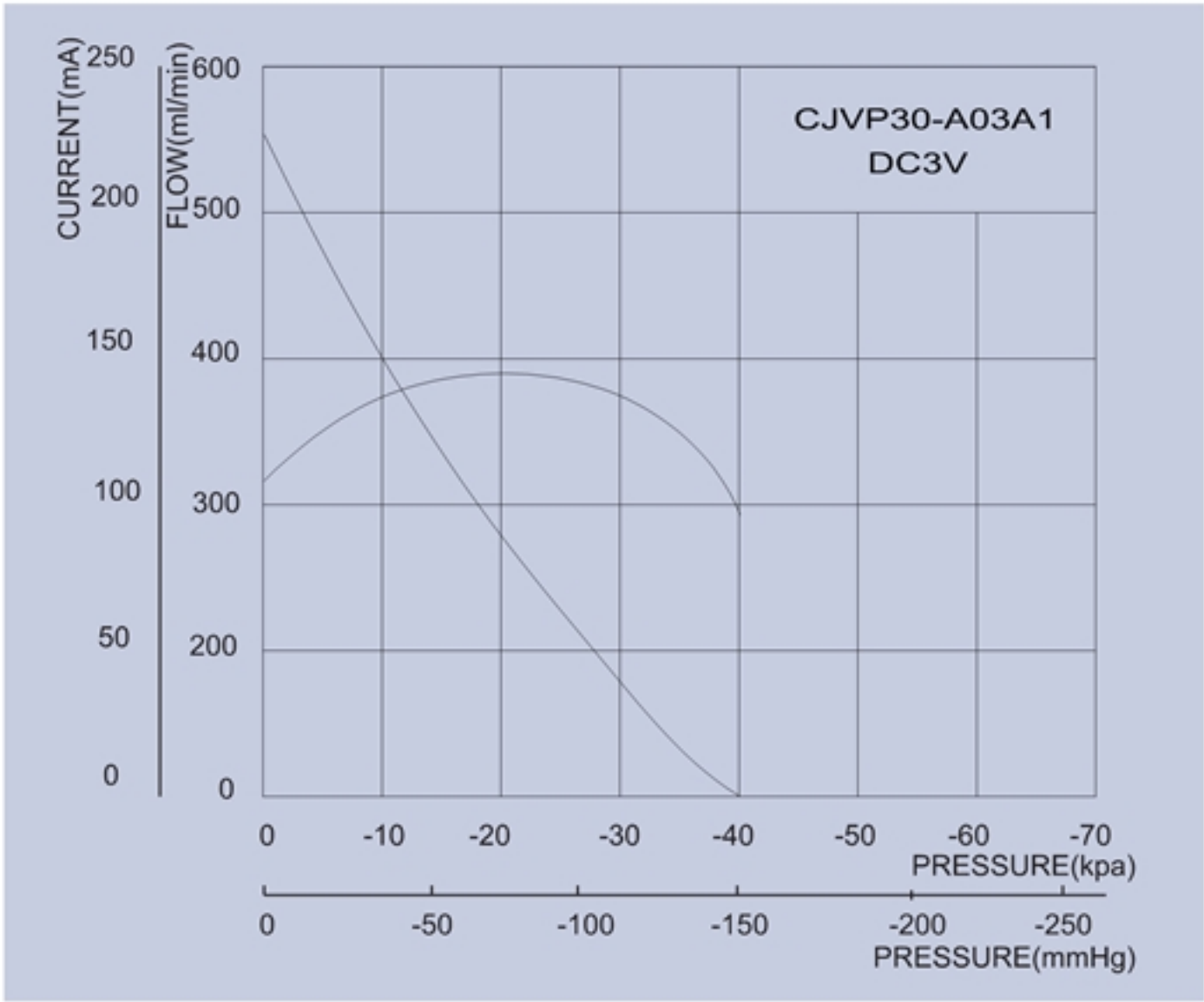
產品特性圖 Performance Curve
