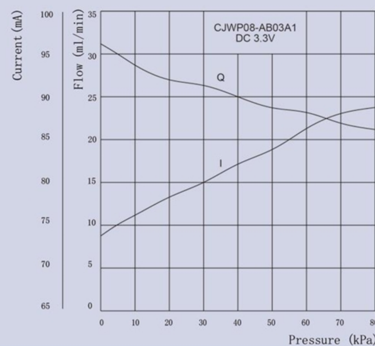
產品特性圖 Performance Curve
