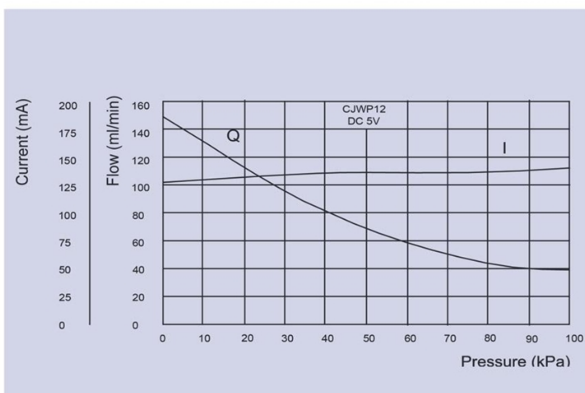
產品特性圖 Performance Curve
